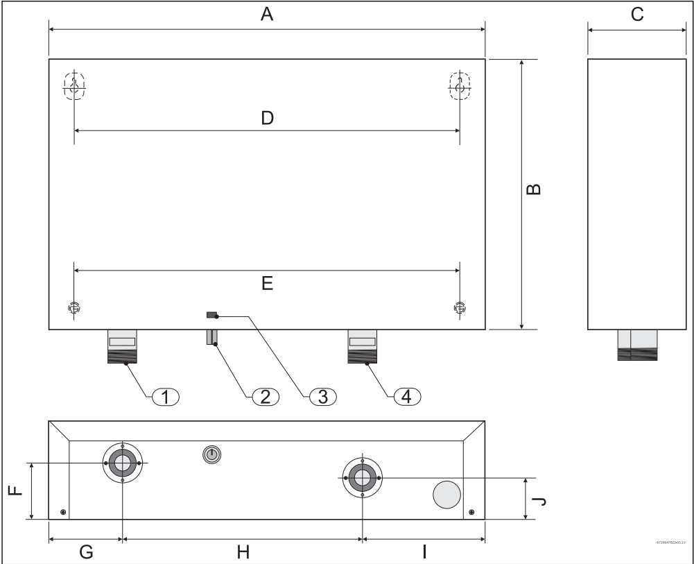
Fig. 2 [1] Sortie ¾ " NPT (eau chaude) [2] Bouton de température [3] LED [4] Inlet ¾ " NPT (eau froide)
