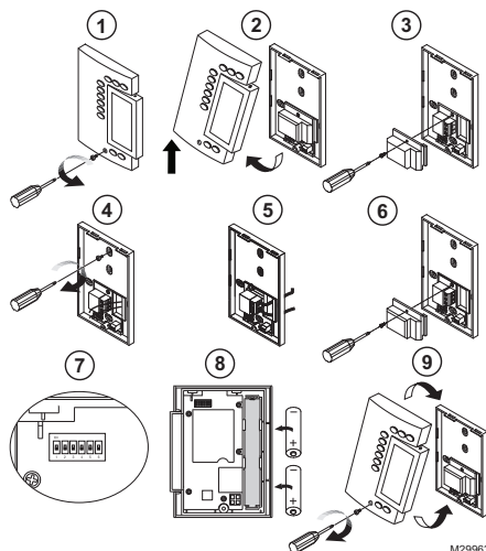
Fig. 1. Installation steps.
