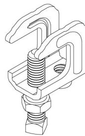
FIG. 345 STAMPED STEEL TOP BEAM CLAMP PAGE 42
