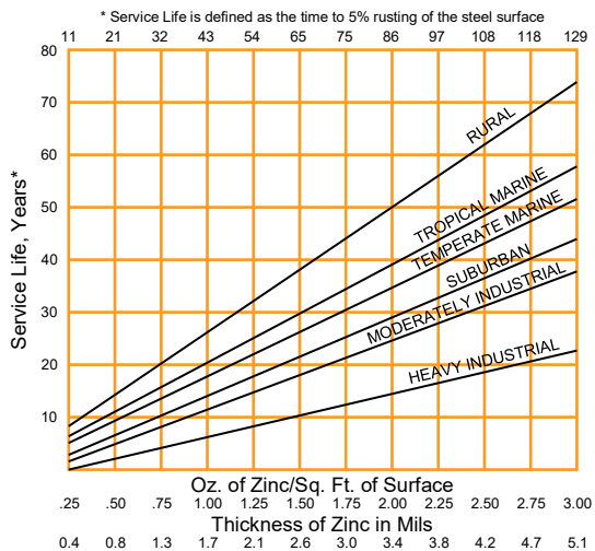
Life of Protection vs. Thickness of Zinc And Type of Atmosphere
