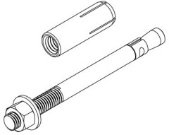
FIG. 47 CONCRETE ANCHORS PAGE 26
