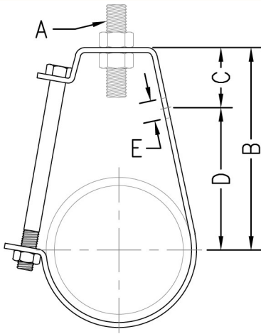
FIG. 970, 970F, & 973
