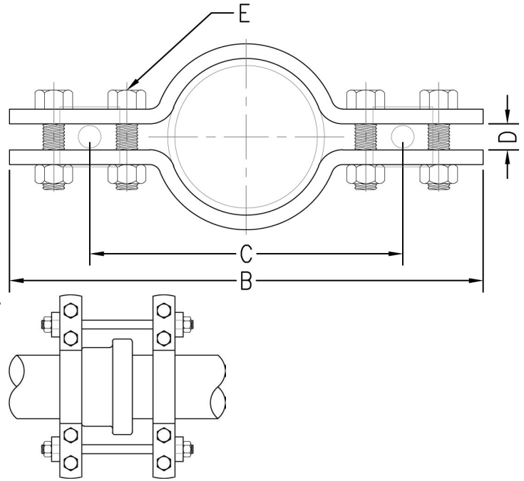
Typical Installation
