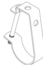
FIG. 970 - 973 J-HANGER PAGE 56
